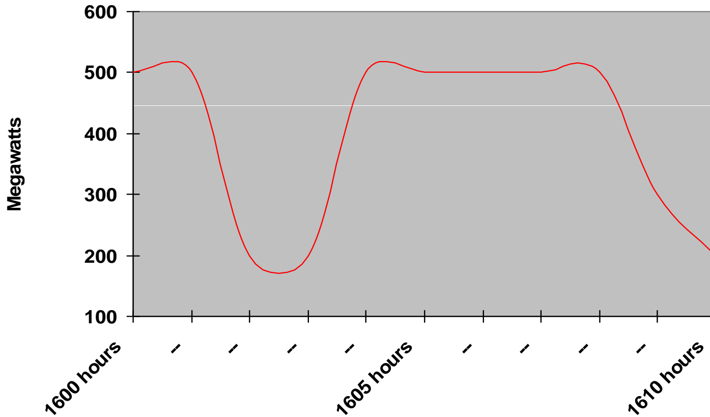
Photovoltaic Array – Partly-Cloudy-Day Generation
