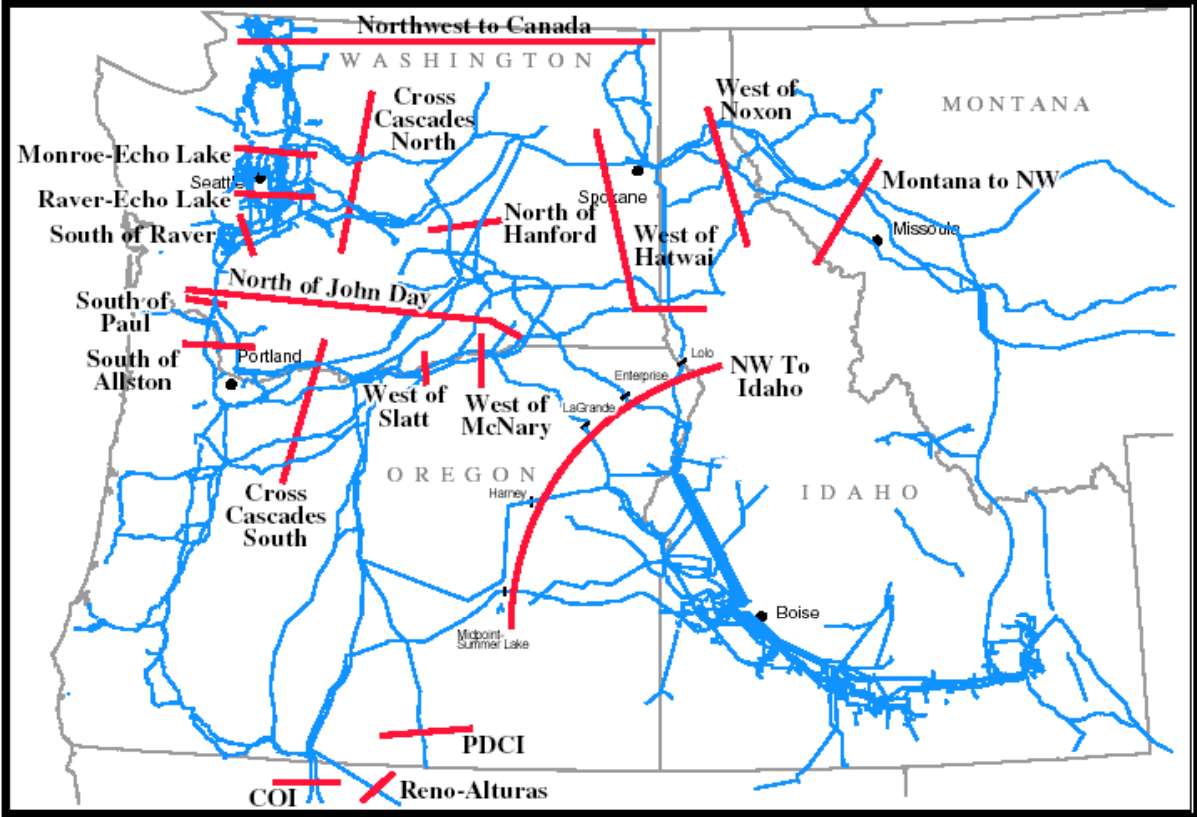
Northwest Transmission Cut Planes
