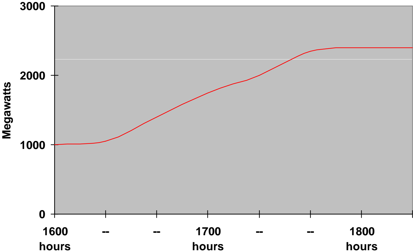
Wind Generation – Weather Front Moving Through
