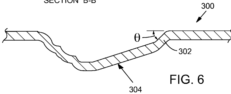
SECTION B-B
